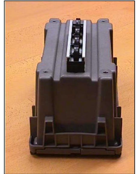
EF-2047D (Above) Typical Container with guidance groove (right)
